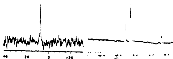
Fig.1: Left, in vivo ^{19}\text{F} NMR spectra in VX2 tumor of rabbit. Right: spectra following excision.
