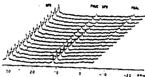
Serial ^{19}\text{F} NMR spectra of the fluorinated compounds in the Walker 256 of the rat following administration of 5FU, either alone or following prior 12 hr administration of methotrexate. Each spectra is a collection of 1024 FID's collected over a 10 min period. Top panel: 5FU alone; bottom panel: 5FU given 5 hrs after a dose of methotrexate. 5FU = 5-fluorouracil; FNUC = fluorinated nucleosides/nucleotides; FBAL = fluoro-beta-alanine; 5FU = 1,2-difluoromethane
