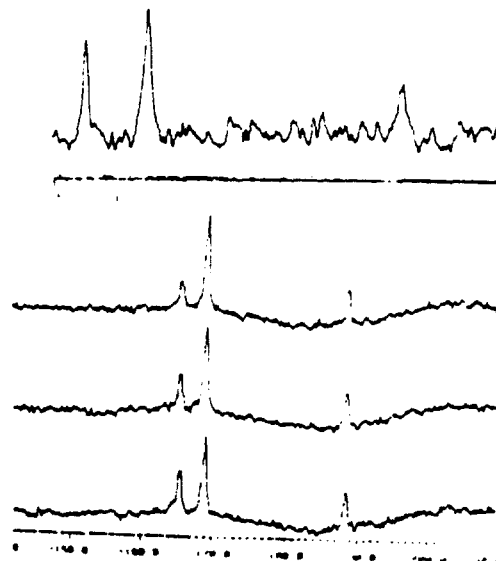
Figure 2: Top, in-vivo ^{19}\text{F} NMR spectra in Walker-256 tumor in rat. Bottom, spectra at 0, 3 and 5 hrs. excised.
