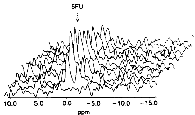
FIG. 2. Stacked plot of ^{19}\text{F} NMR spectra taken over the liver metastasis of the colon carcinoma of patient 6 from 0 to 55 min after i.v. administration of 5FU at 600 mg/m 2 as a bolus. The patient was positioned in a 1.5-T Magnetom before injection. Each spectrum was the result of 256 FIDs acquired at 10-kHz spectral width with the 90° pulse optimized for 4 cm at 60.012500 MHz and a 1-sec repetition rate. All spectra were corrected for baseline and smoothed with a gaussian filter matched to the T_2^* of the FID. Series of consecutive spectra, each collected over a 4.17-min period, were obtained during the first hour after drug administration.
